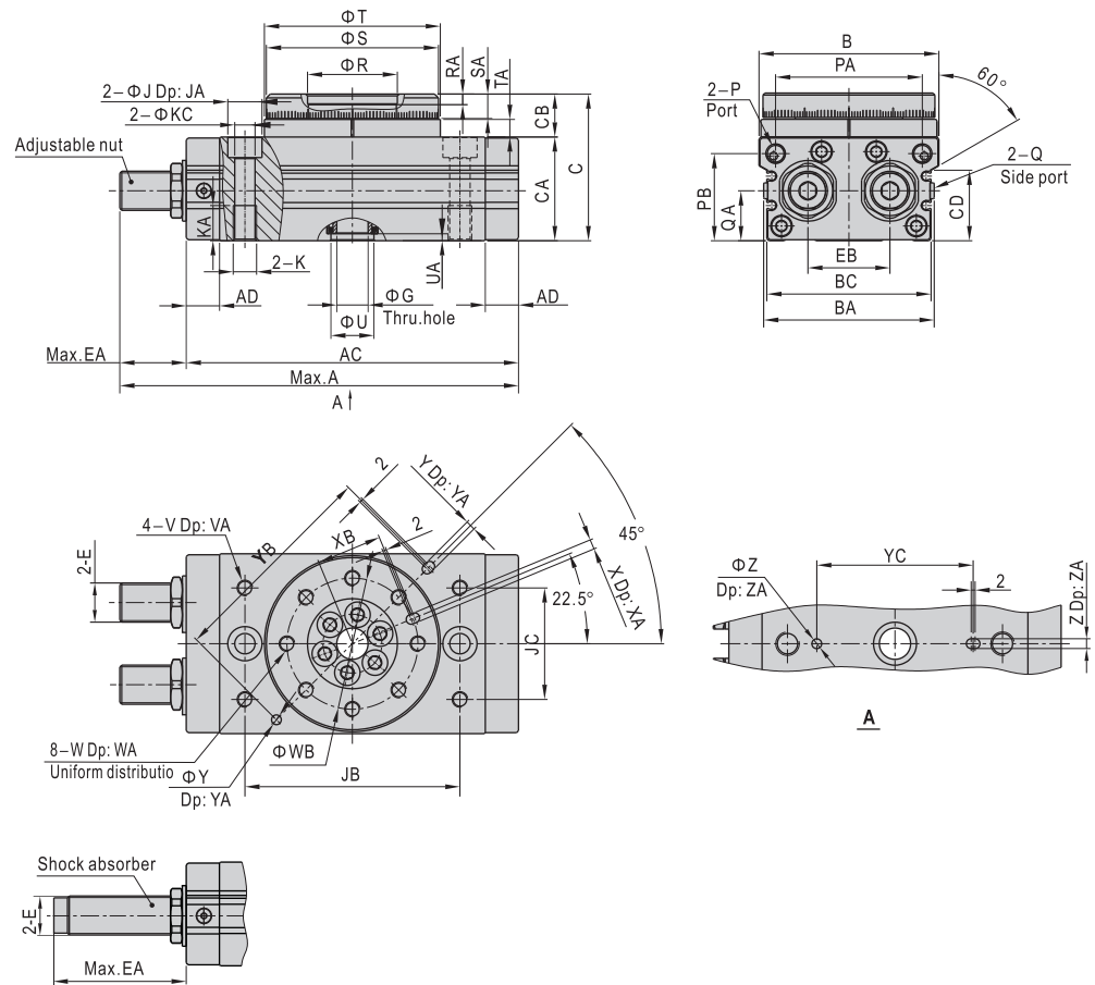
HRQ□-A (With internal shock absorber)
